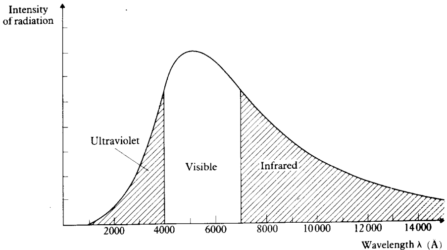
14.15 The spectral distribution of radiation from the sun corresponding to a surface temperature of about 6000 K.
